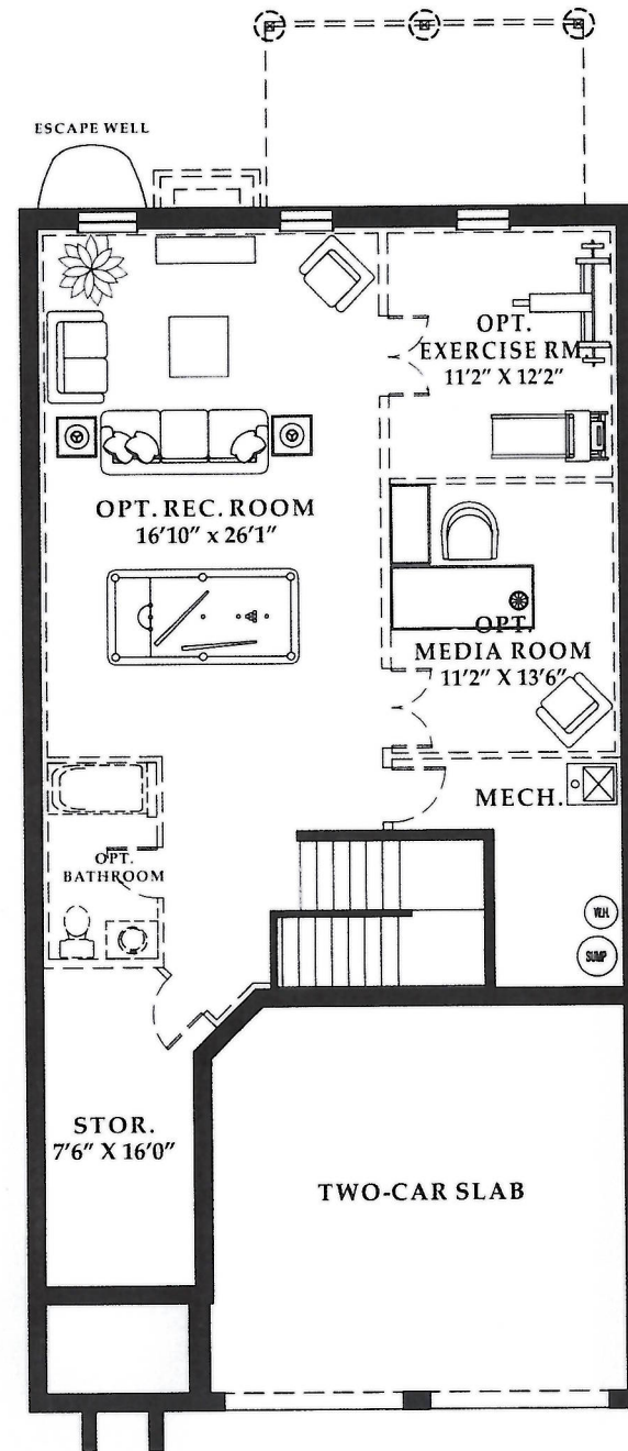
Basement Floor Plan Interior Unit with Optional 10' Extension
